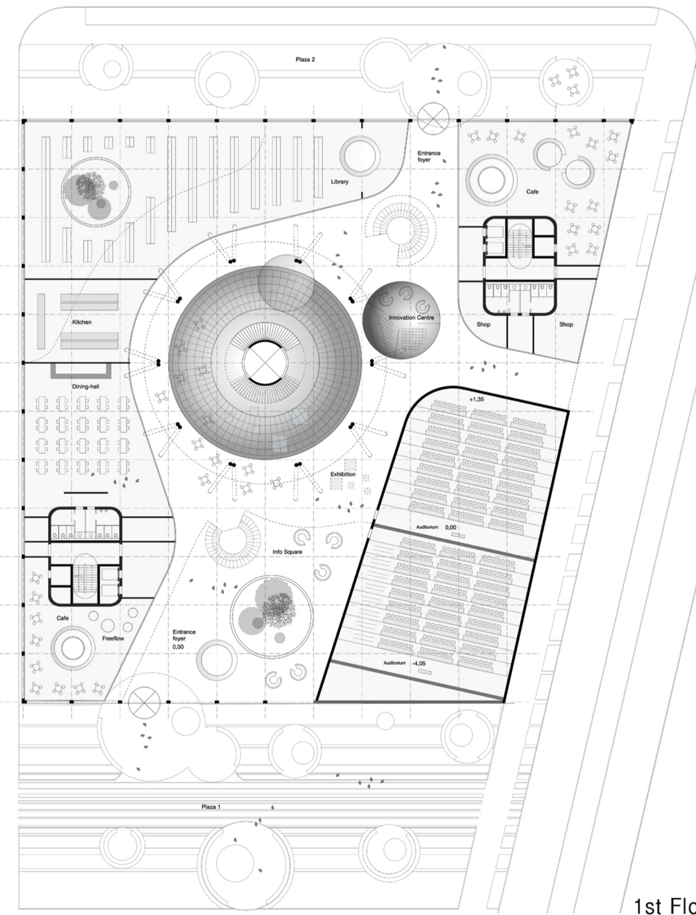
1st Floor
