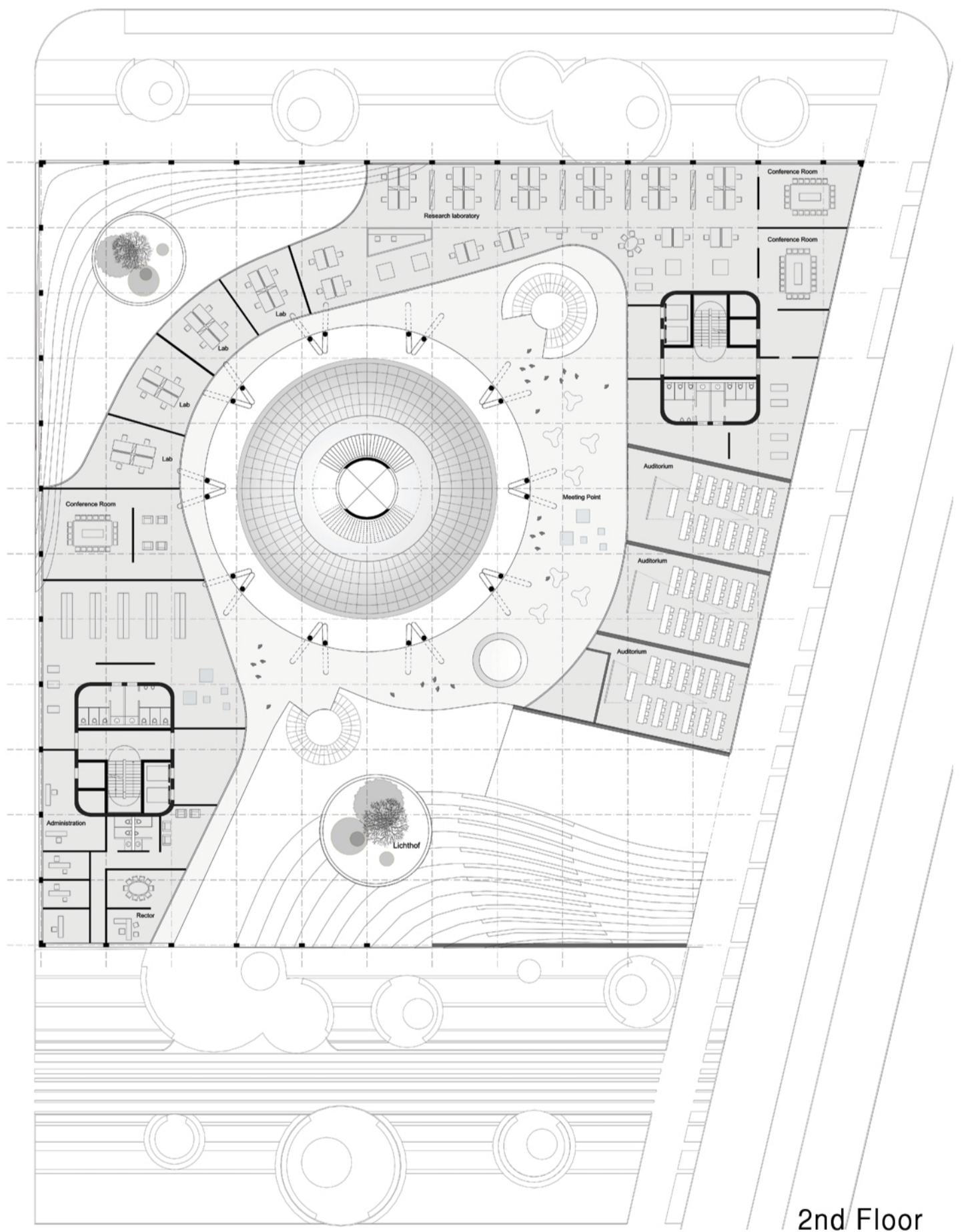
2nd Floor
